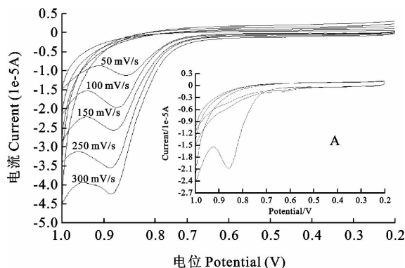
Scan rate (V/s, from top to bottom): 0.050, 0.100, 0.150, 0.250 and 0.300. Accumulation time:240 s. Other conditions as in Fig. 3. Inset: the successive cyclic voltammogram of MG at the FCCBPE (Scan rate:0.100 V/s)
